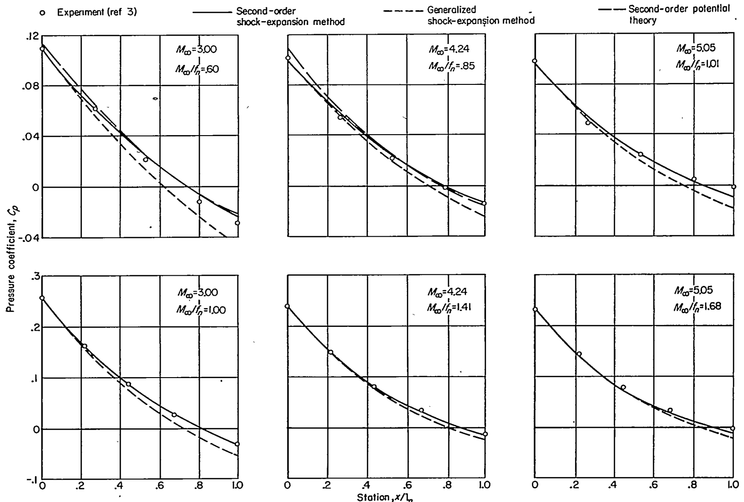
FIGURE 6.—Surface-pressure distributions for noninclined tangent ogives.
