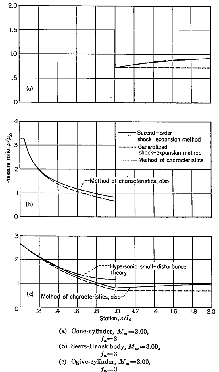
FIGURE 5.—Surface-pressure distributions for various bodies at M_\infty/f_n=1 and \alpha=0 .
