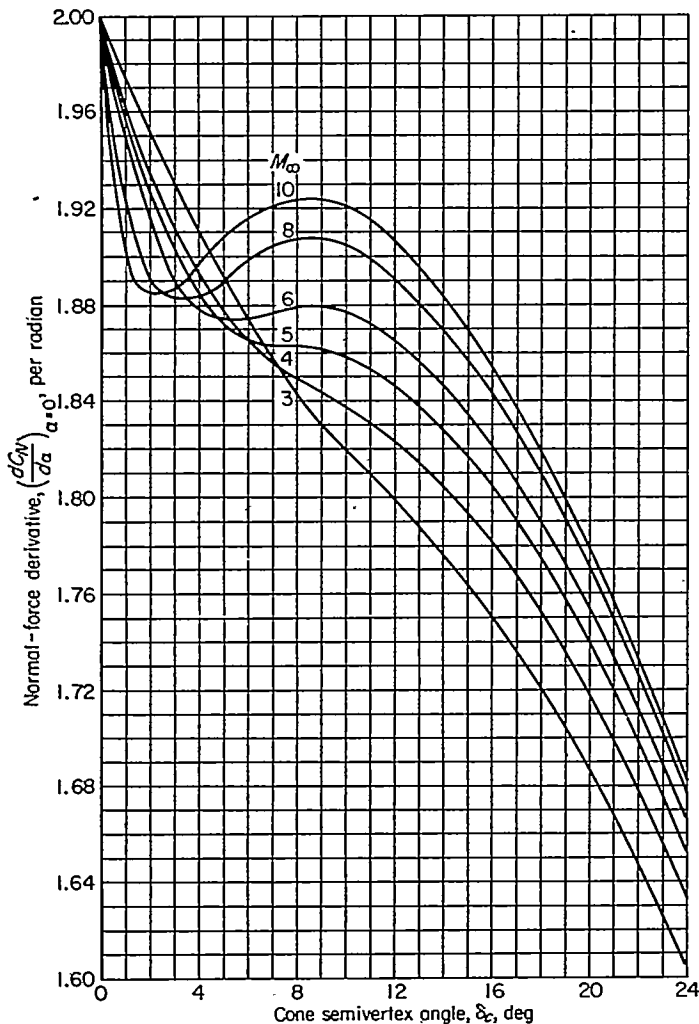
FIGURE 4.—Normal-force derivative \left( \frac{dC_N}{d\alpha} \text{ at } \alpha=0 \right) for cones (ref. 14).
