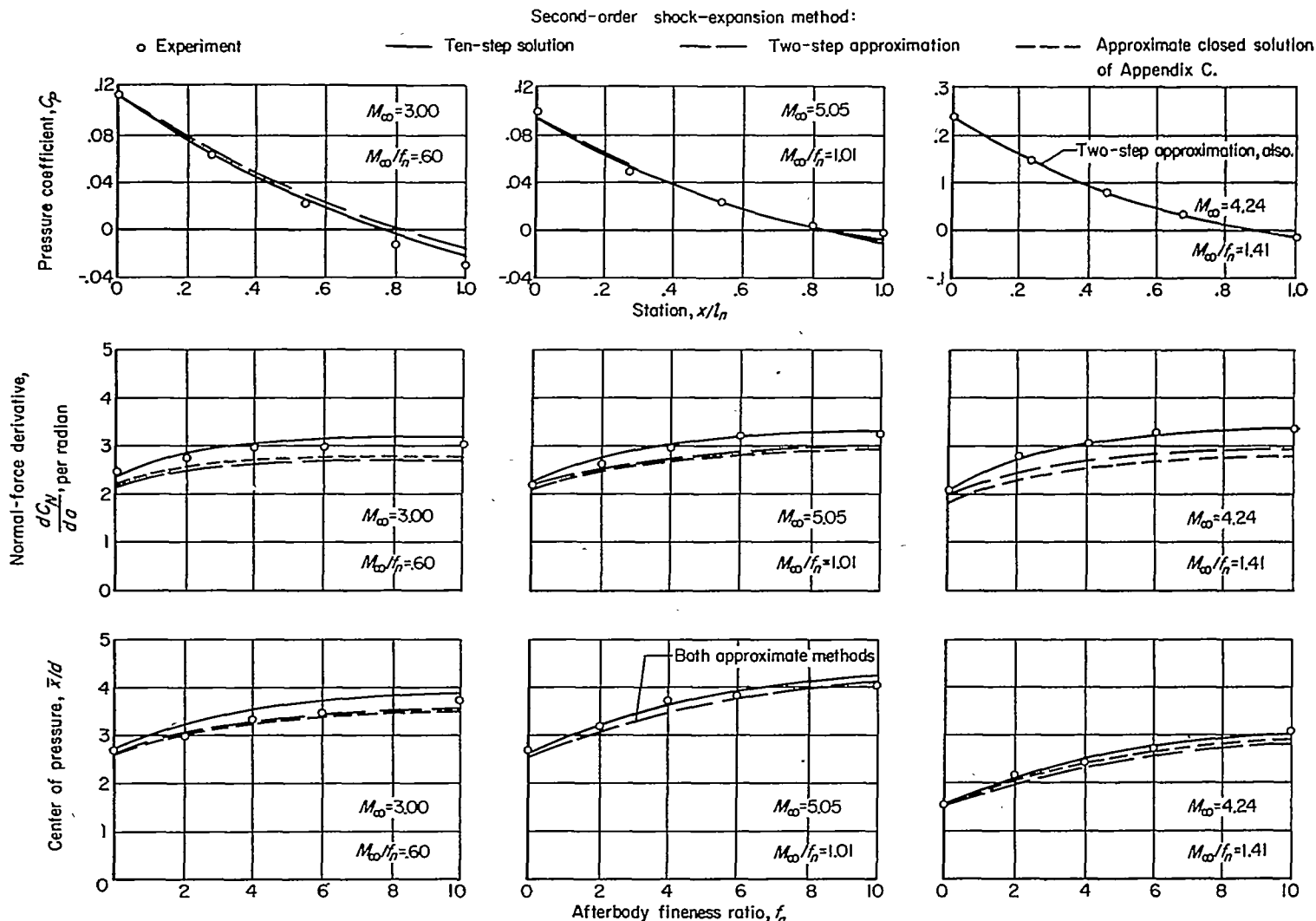
FIGURE 9.—Accuracy of approximate solutions for ogive-cylinders ( \alpha=0 ).
