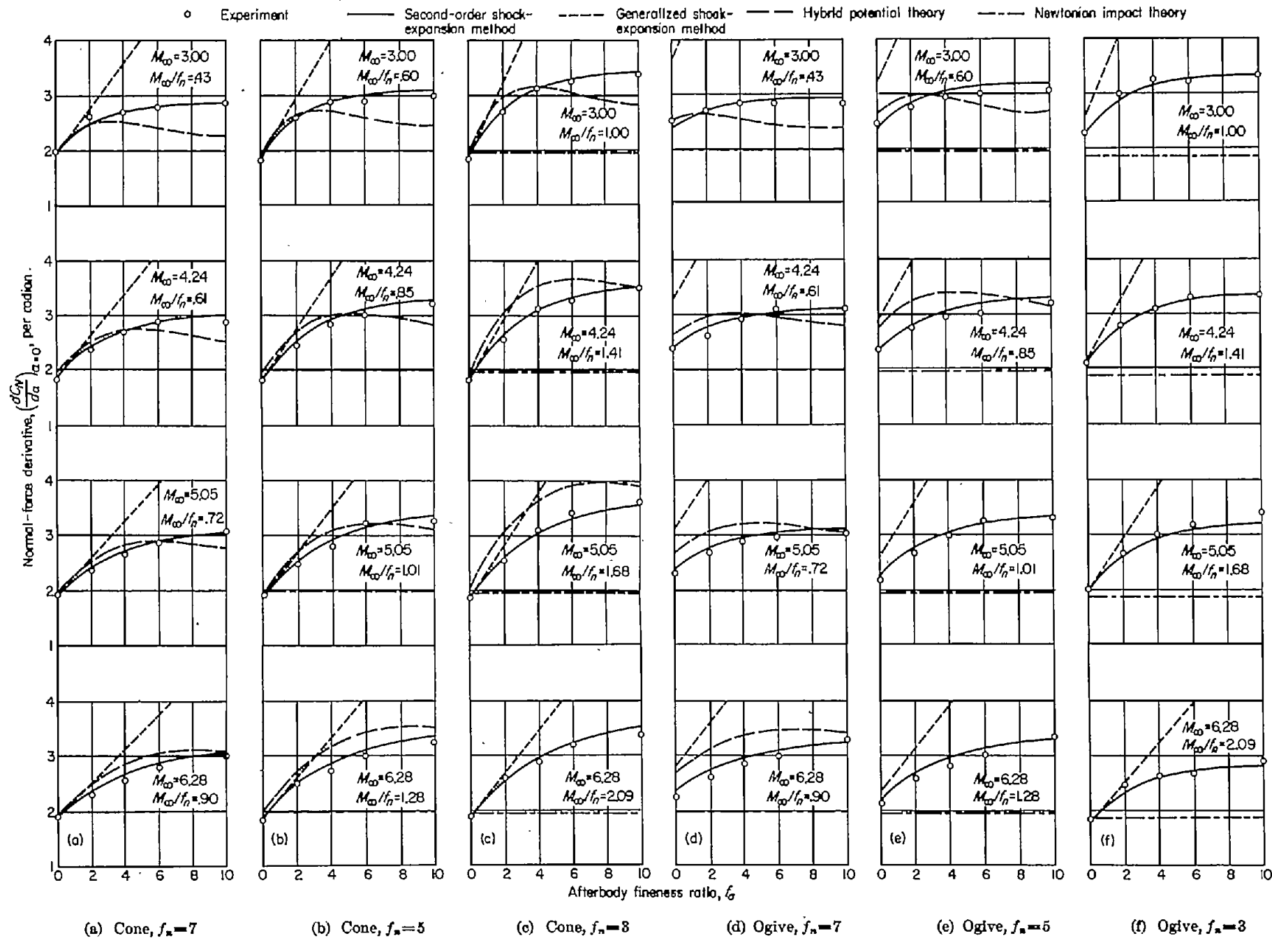
FIGURE 7.—Normal-force derivatives for various cone- and ogive-cylinders at Mach numbers from 3.00 to 6.28.
