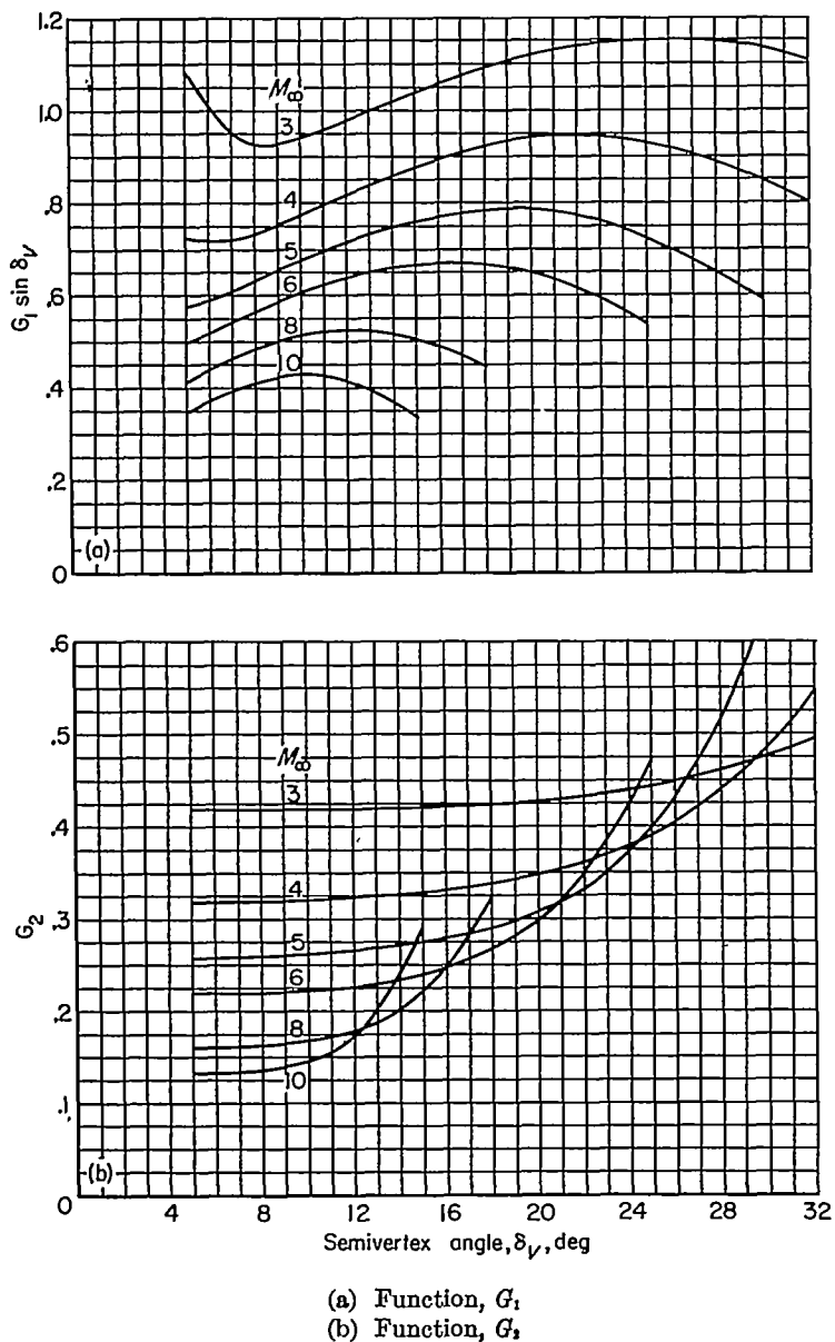
FIGURE 12.—Curves defining functions G_1 and G_2 (Appendix C).
