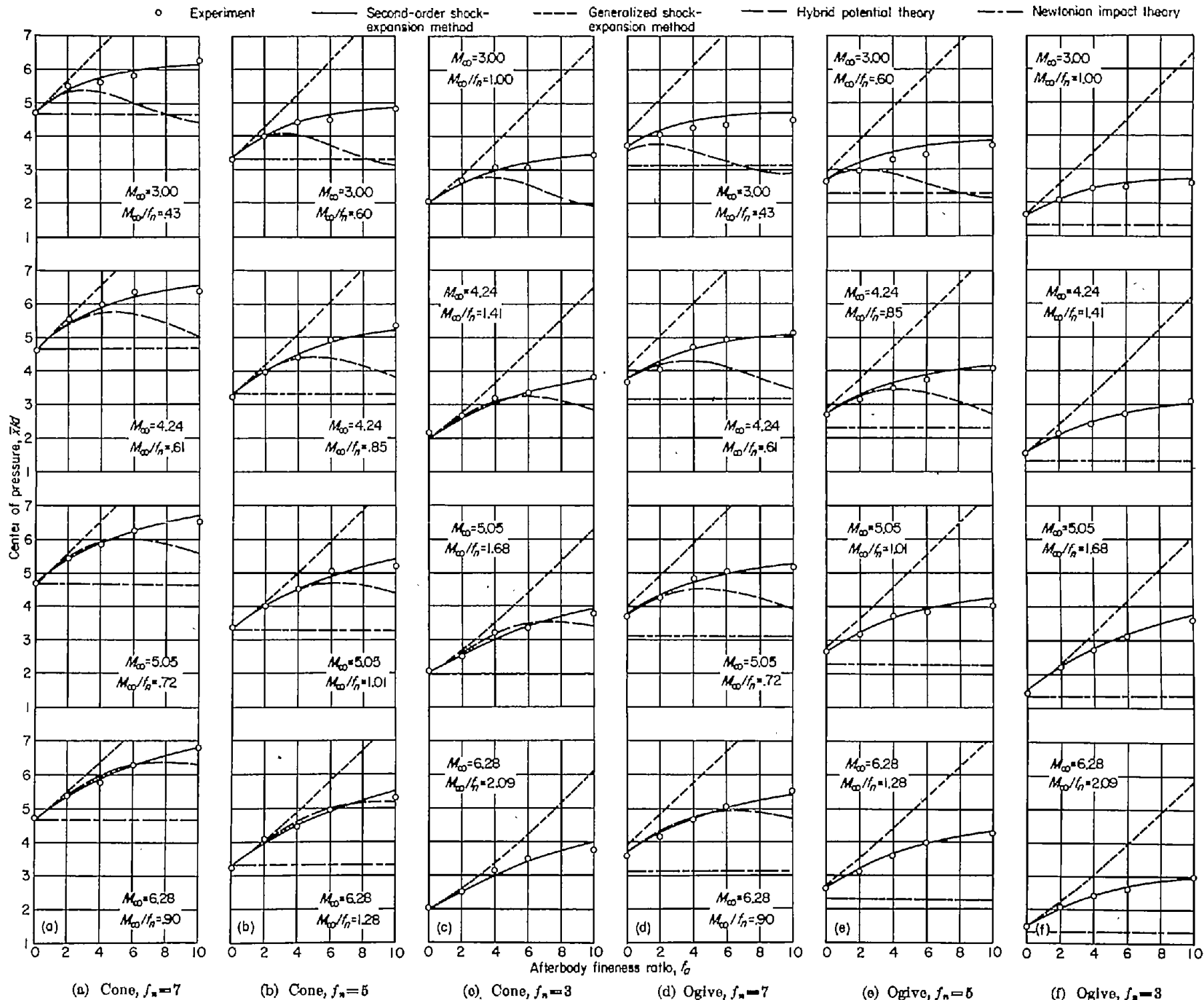
FIGURE 8.—Centers of pressure at \alpha=0 for various cone- and ogive-cylinders at Mach numbers from 3.00 to 6.28.
